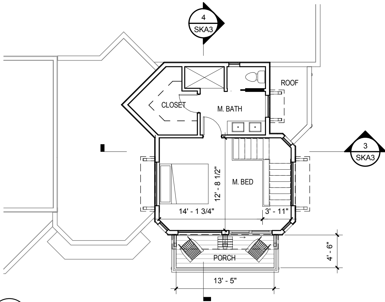
2 2nd FLOOR PLAN 1/8" = 1'-0"
